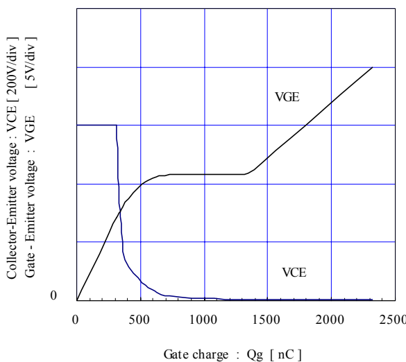
Dynamic Gate charge (typ.) Vce=600V, Ic=450A, Tj= 25°C
